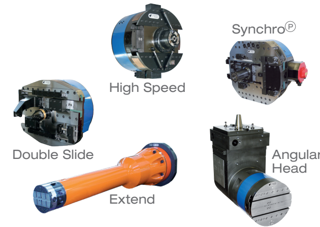
Medium and large NC heads for boring machines and special units
