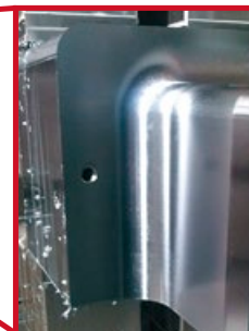
1ワーク88m(3時間)加工後の刃先の損傷状態 Cutting edge after 88m (3 hours) of milling
